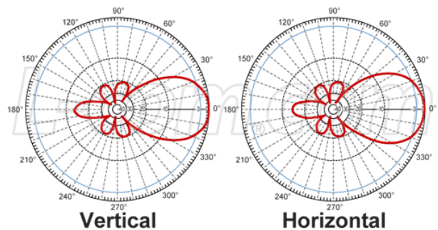
Radiation pattern
