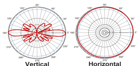
Radiation pattern
