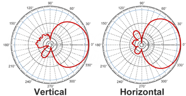
Radiation pattern
