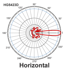
Radiation pattern
