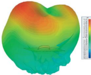
3D Gain Plot Top (5.4GHz)
