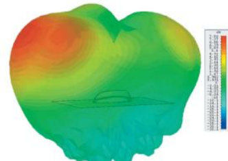
3D Gain Plot Top (2600MHz)
