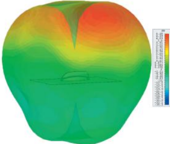
3D Gain Plot Top (800MHz)
