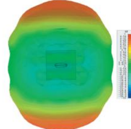
3D Gain Plot Top (2600MHz)
