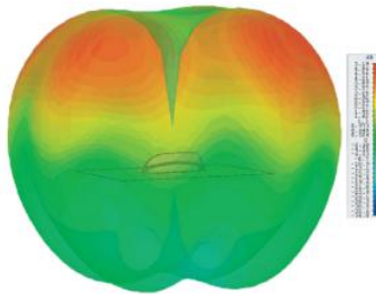
3D Gain Plot Top (1800MHz)
