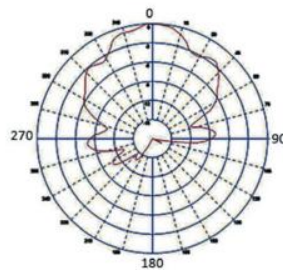
Typical Radiation Patterns - GPS/GNSS Element 1
