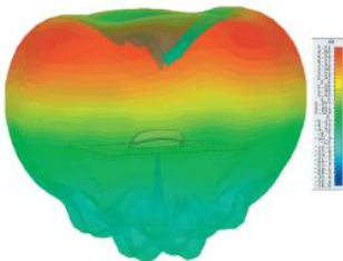
3D Gain Plot Top (2100MHz)
